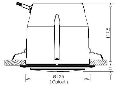
Side View (unit: mm)
