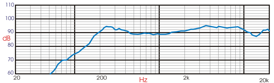
Frequency response
